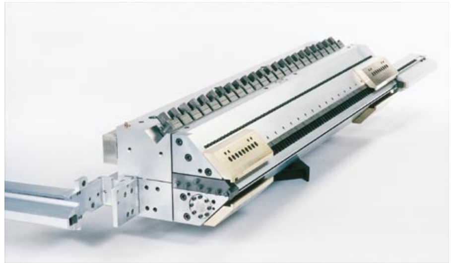
Figure 9. Sheet die with internal deckles (Courtesy of EDI)
