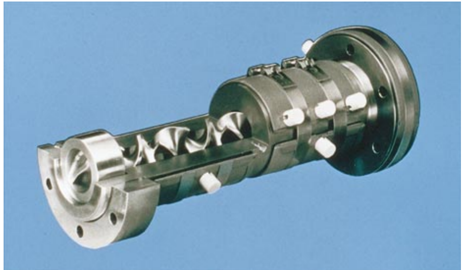
Figure 5. Static mixing sections (Courtesy of Chemineer-Kenics)
